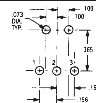
Contacts Make on Opposite Side Toggle Thrown
