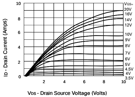
Saturation Characteristics
