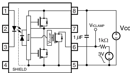
Fig. 10 V tCLAMP Test Circuit
