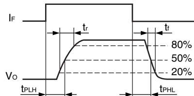
Fig. 7 t_{PLH}/t_{PHL}/t_r/t_f Test Circuit and Wave Forms
