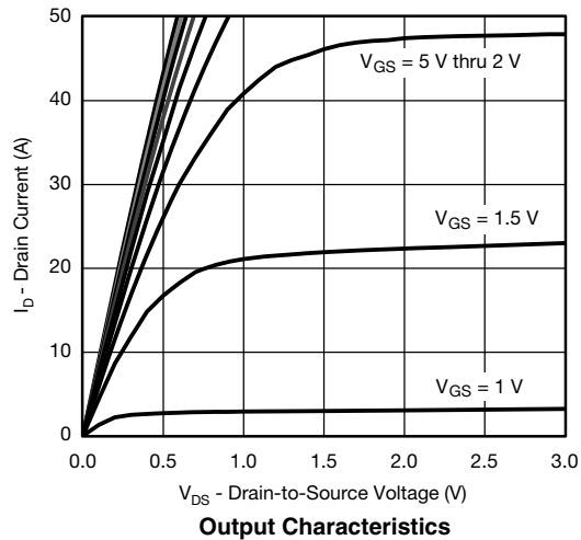
Output Characteristics
