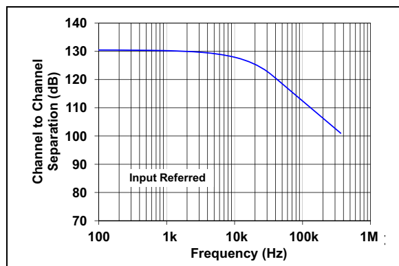
FIGURE 2-19: Channel-to-Channel Separation vs. Frequency (MCP6H72/4 only).
