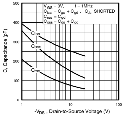
Fig 19. Typical Capacitance Vs. Drain-to-Source Voltage
