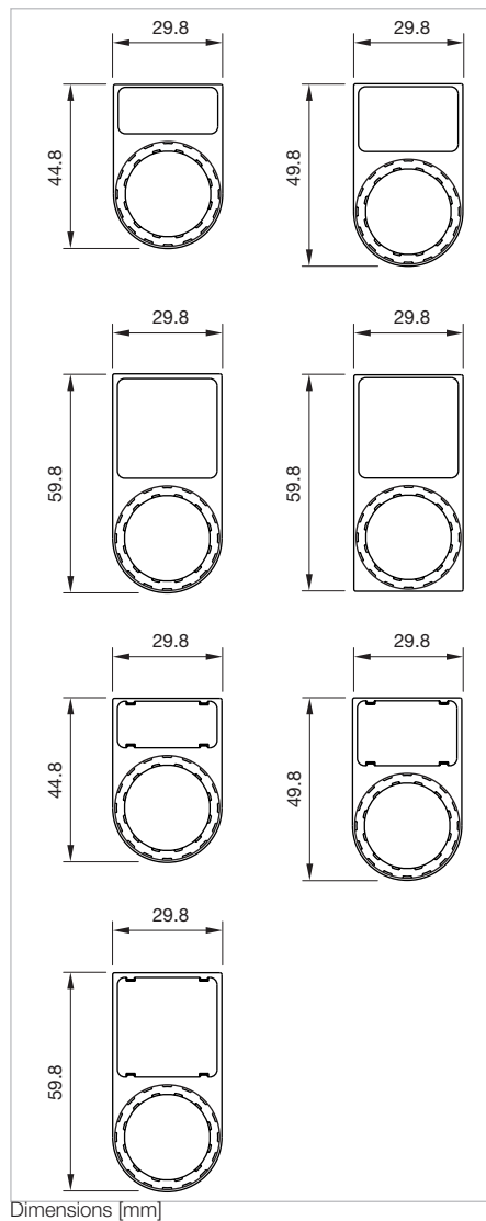
Dimensions [mm]
