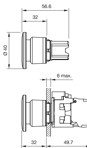
Mushroom-head pushbutton Momentary/Maintain, Momentary/Momentary, Ø 40 mm (raised design)
