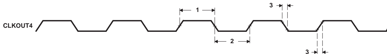
Figure 5-12. CLKOUT4 Timing
