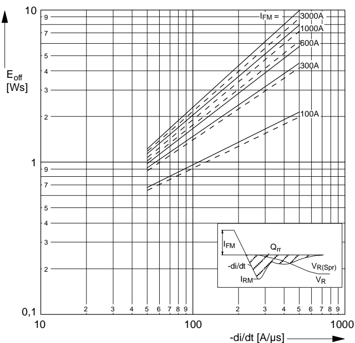
Fig. 12 Turn-off-losses E_{off} = f(di/dt) diodes with V_F max Application: GTO-freewheeling diode Parameter: I_{FM} : Snubberdiode D 291 S t_{vj} = 125^\circ\text{C} ; C_S = 4 \mu\text{F} für V_R \leq V_{RM} C_S = 24 \mu\text{F} für V_R \geq V_{RM} L_S = 0,2 \mu\text{H}
