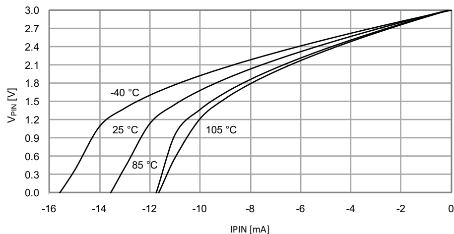
Figure 36-22. I/O Pin Output Voltage vs. Source Current
