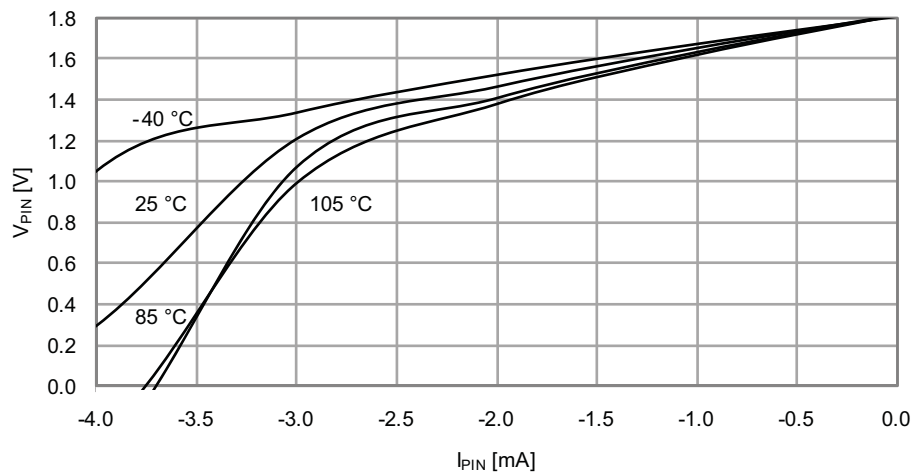
Figure 36-21. I/O Pin Output Voltage vs. Source Current
