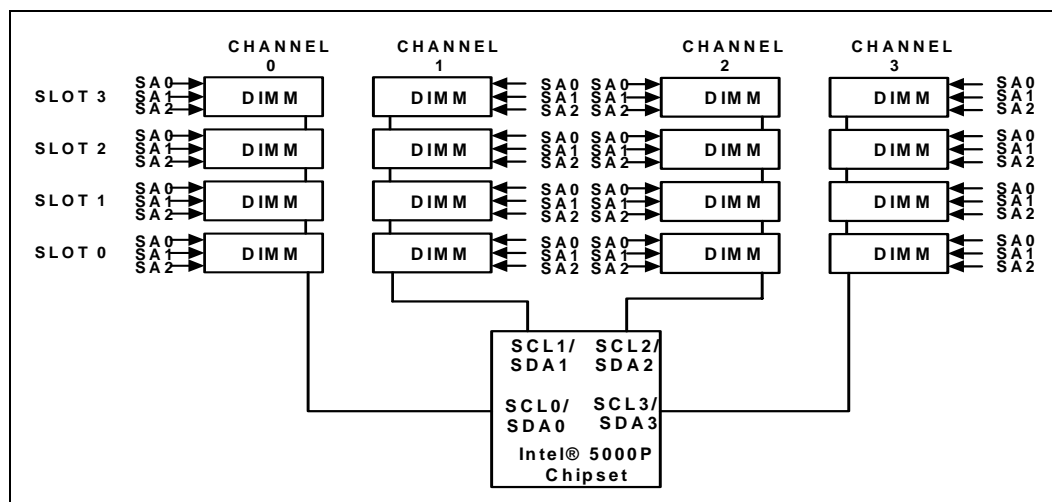
Figure 5-8. Connection of DIMM Serial I/O Signals
