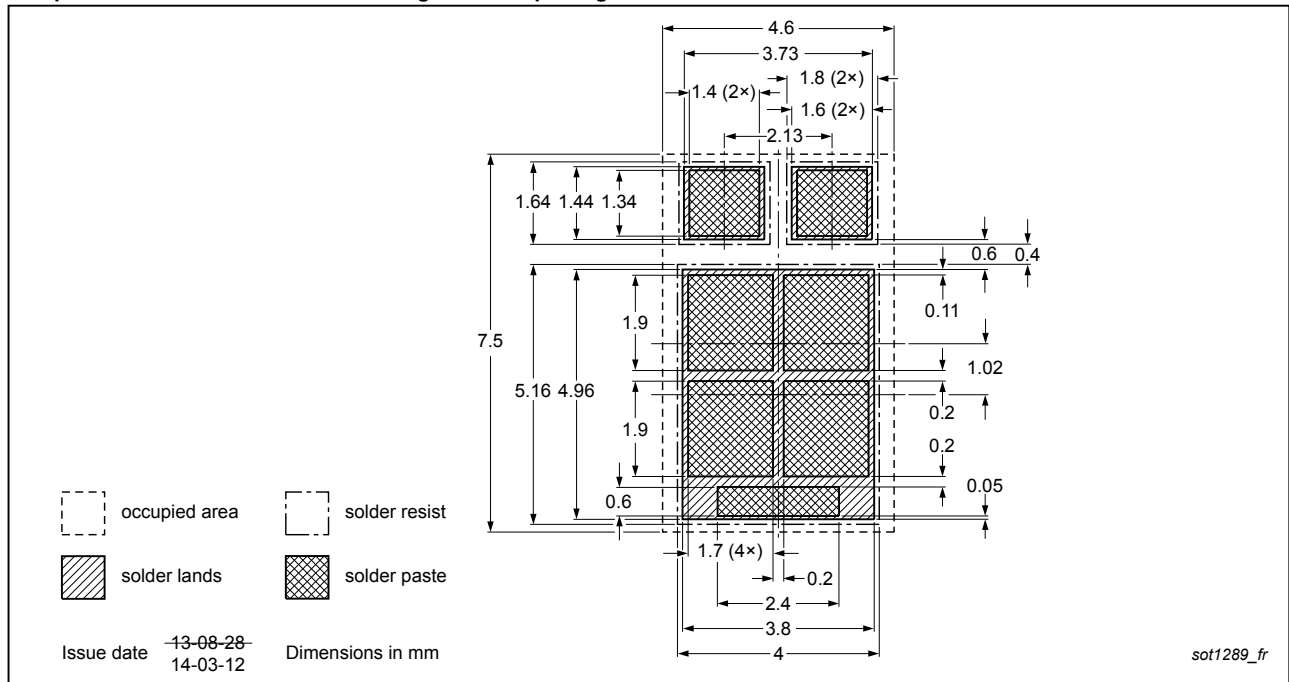
Fig. 18. Reflow soldering footprint for CFP15 (SOT1289)
