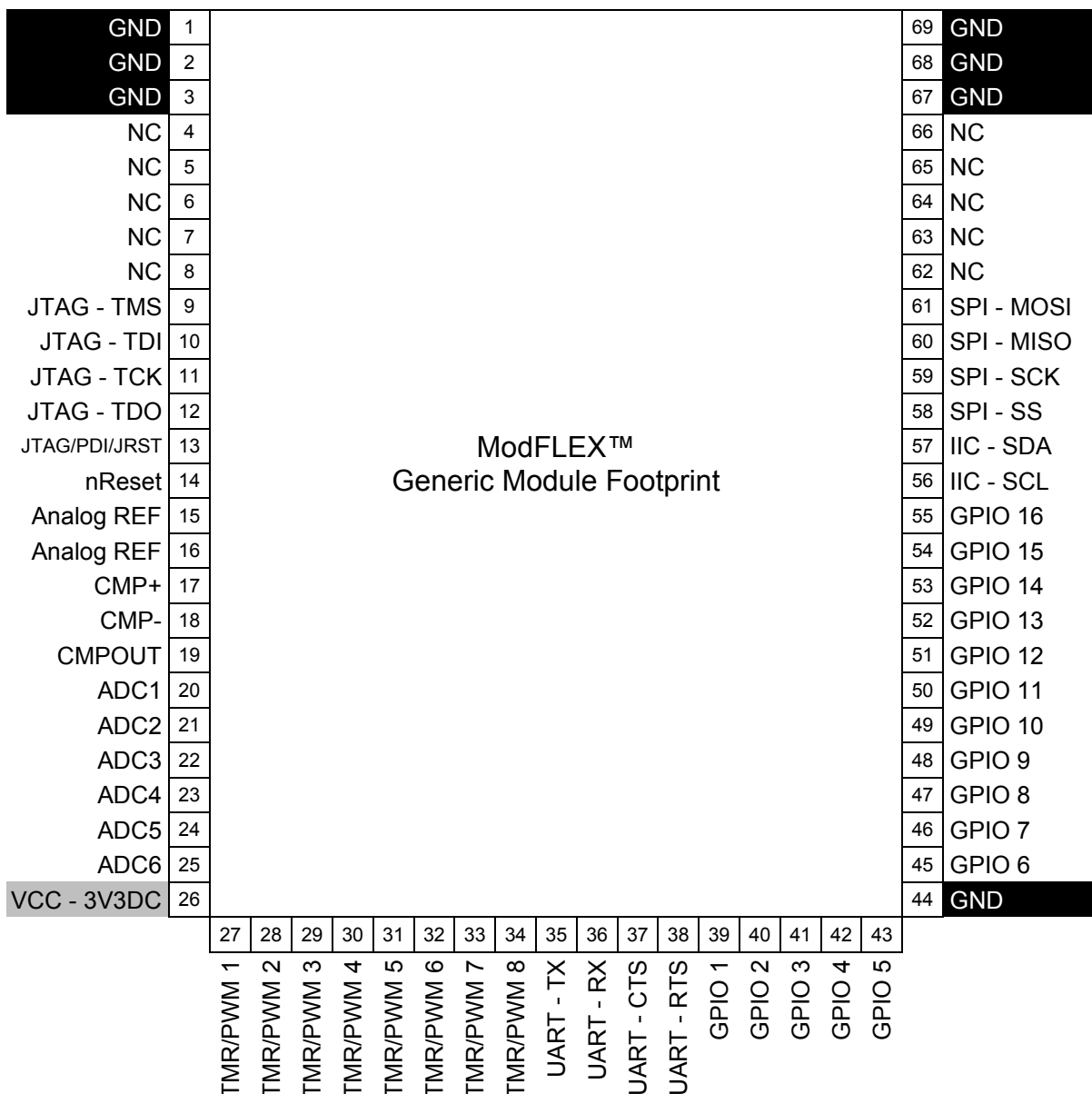
Figure 18 ModFLEX™ Generic Module Footprint
