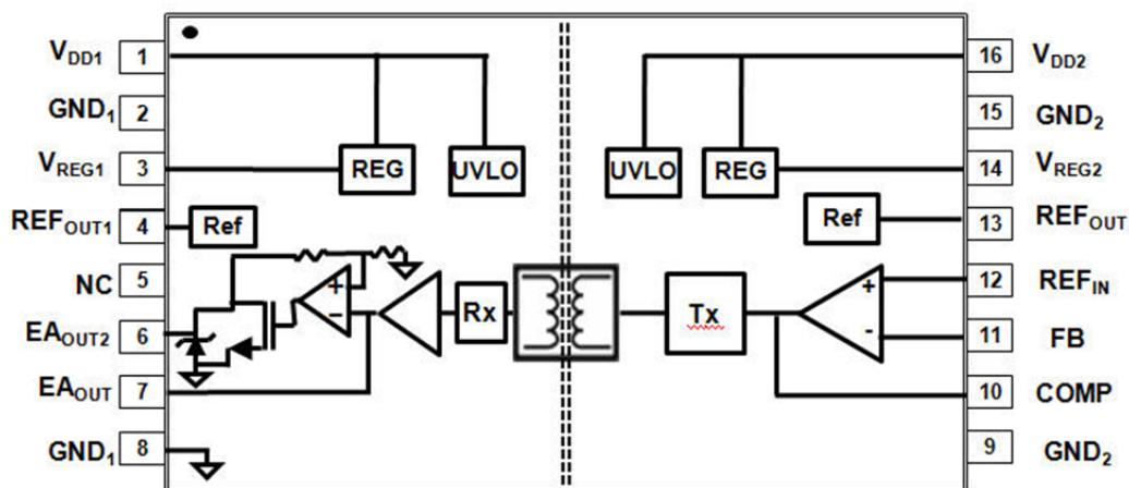
Figure 3. ADuM3190 Block Diagram
