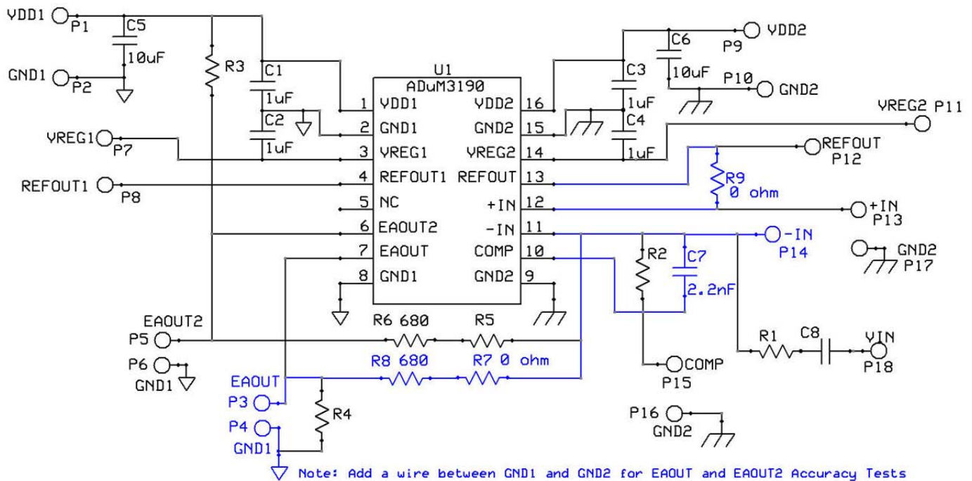
Figure 2. EVAL-ADuM3190EBZ Schematic
