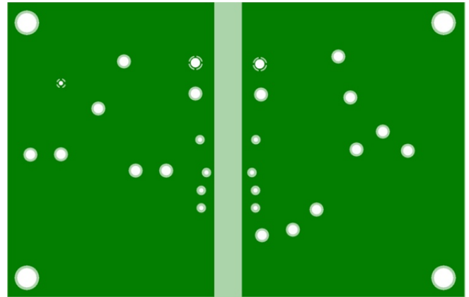
Figure 6. Layer 3: Power Plane
