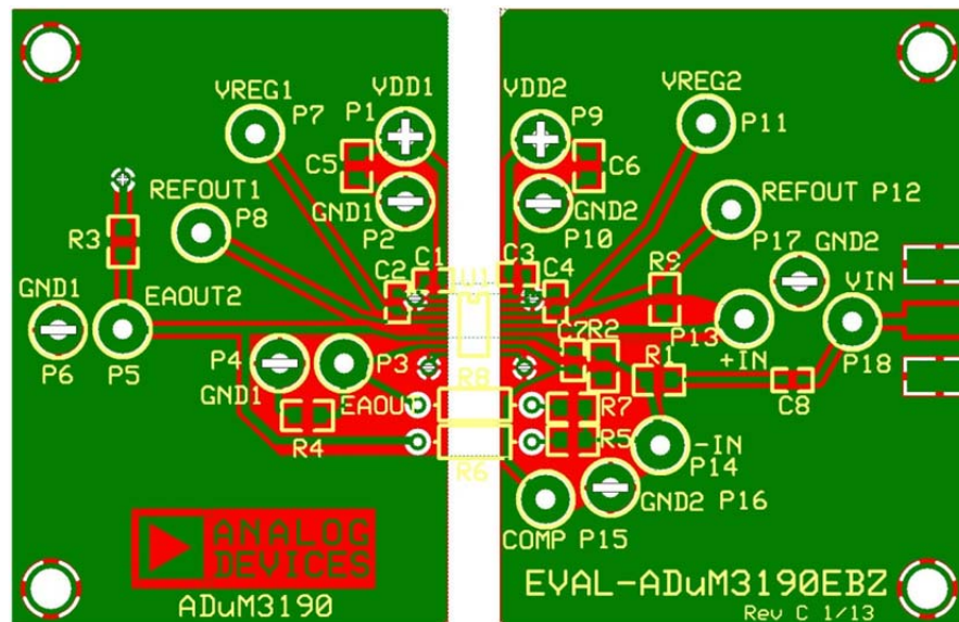
Figure 1: EVAL-ADuM3190EBZ (add photo- available in about 2 weeks)
