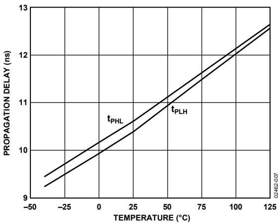
Figure 7. Typical Propagation Delays vs. Temperature, 5 V Operation
