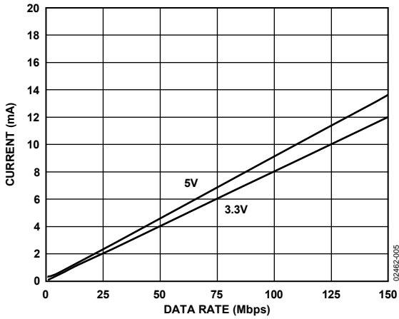
Figure 5. Typical Input Supply Current vs. Logic Signal Frequency for 5 V and 3.3 V Operation
