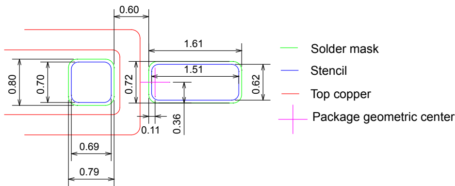
Figure 16: Recommended PCB solder pad layout for LUXEON 3014.
