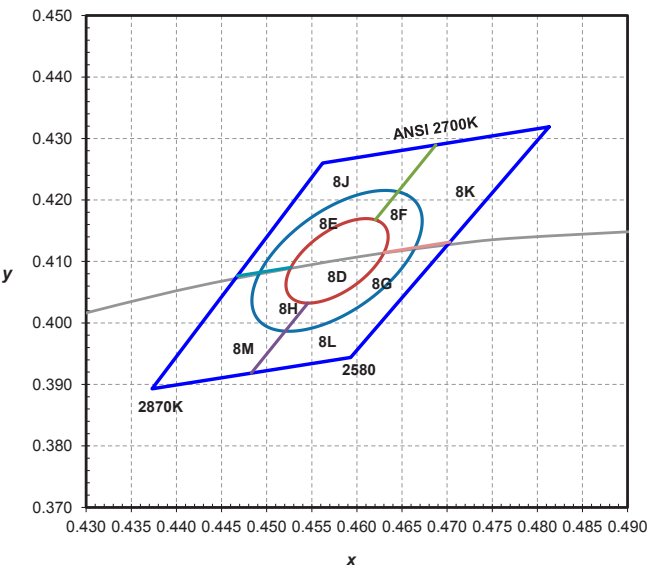
Figure 7: Color bin structure for LUXEON 3014 2700K.
