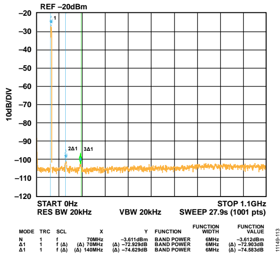
Figure 102. Single Carrier at 70 MHz Output
