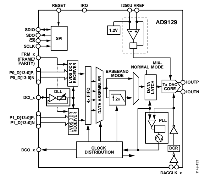
Figure 128. Functional Block Diagram of the AD9119/AD9129
