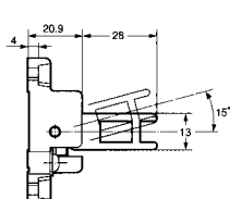
Horizontal/Vertical-adjustable Vertical Mounting
