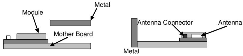
Figure 8 Recommended Locations in z-plane
