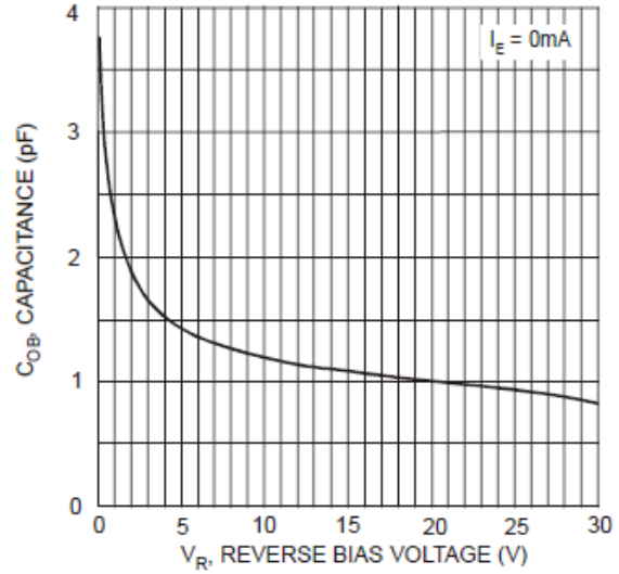
Fig. 4 Output Capacitance
