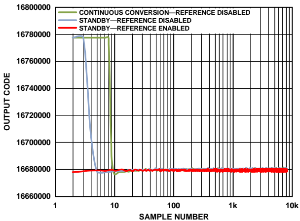
Figure 19. Internal Reference Settling Time
