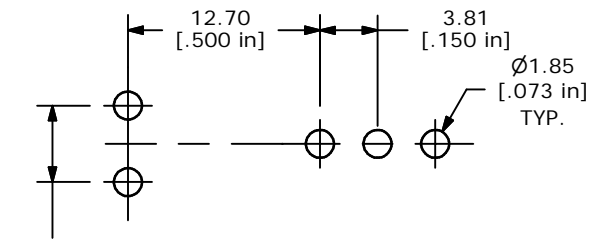
RECOMENDED PC MOUNTING
