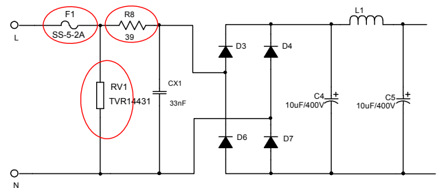
Figure 9: Solution to Pass 2kV Surge Test Layout Guide
