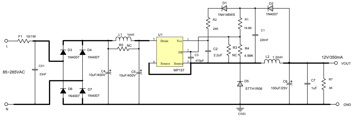
Figure 11: Typical Application at 12V, 350mA
