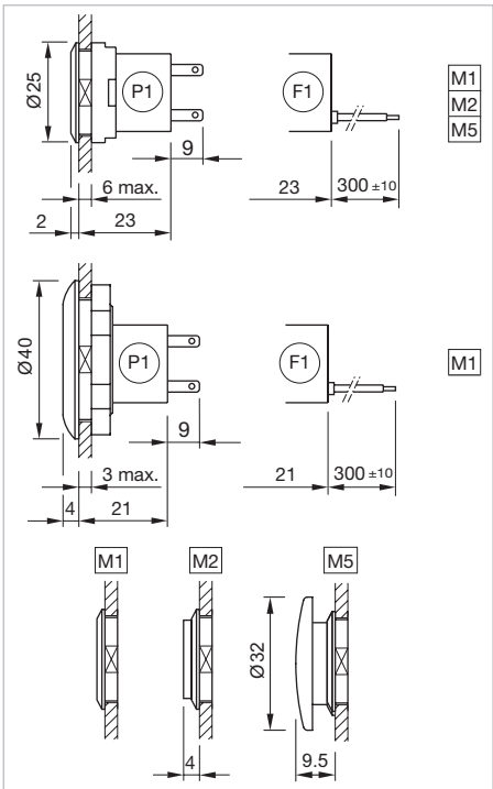
Dimensions [mm] F1 = Flat ribbon cable, P1 = Plug-in terminal 2.8 x 0.8 mm, M1 = Lens level with bezel, M2 = Lens raised above bezel, M5 = Mushroom-head cap
