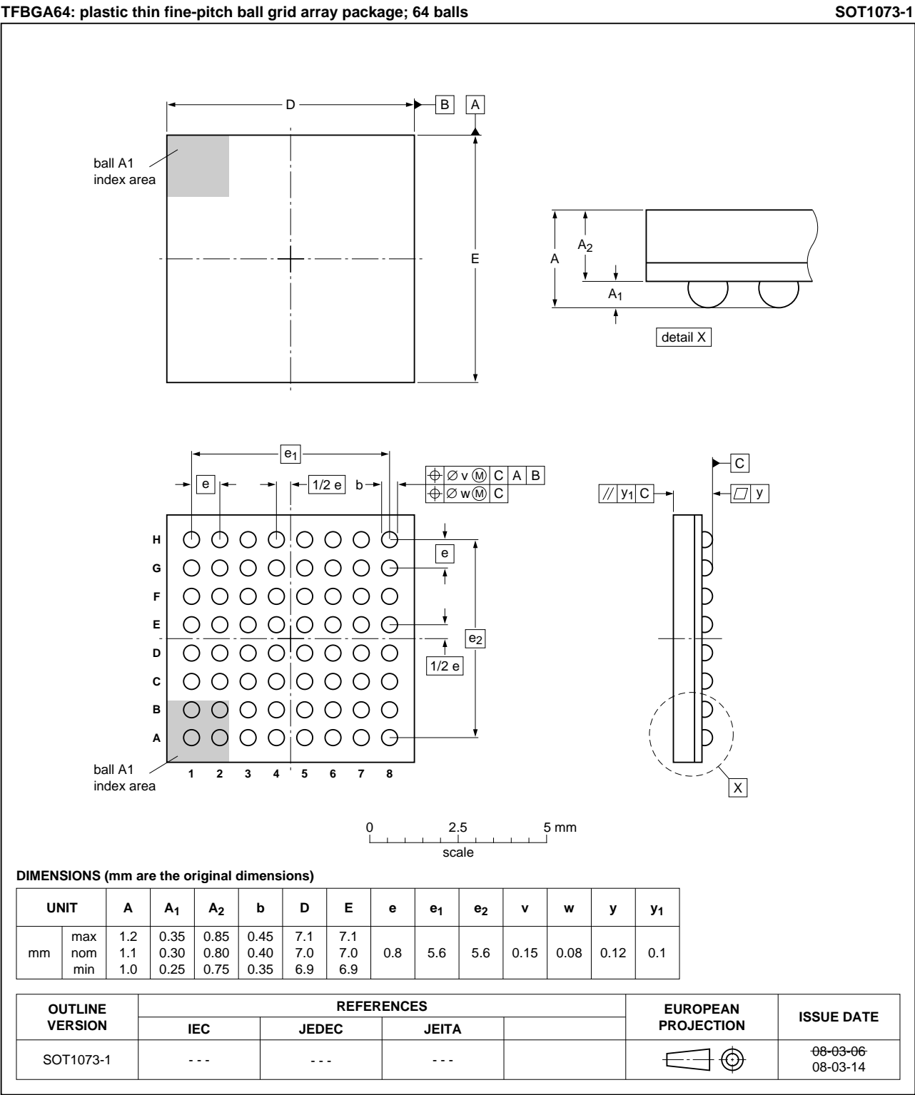
Fig 15. Package outline SOT1073-1 (TFBGA64)
