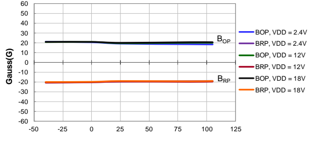
Magnetic Switch Points Bop & Brp vs. Temperature
