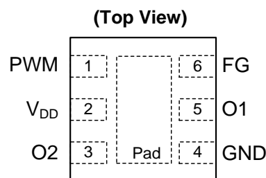
U-DFN2020-6
