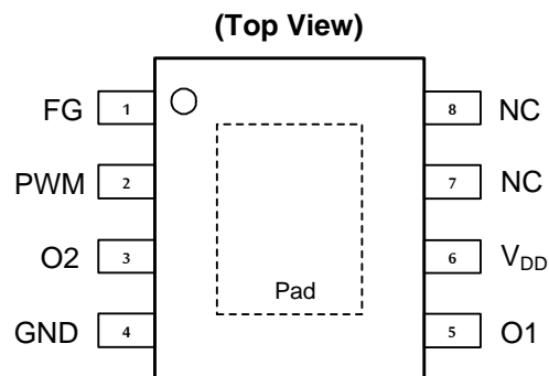
MSOP-8EP
