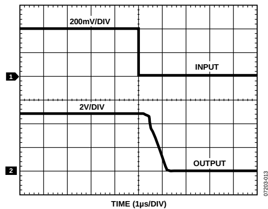
Figure 15. Differential Overload Recovery (Falling)
