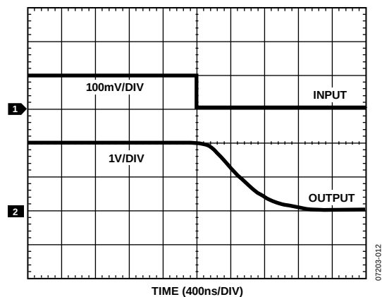
Figure 13. Fall Time
