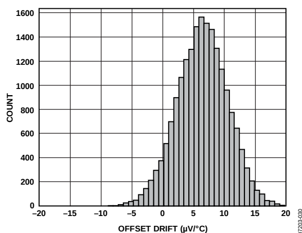
Figure 25. Offset Drift
