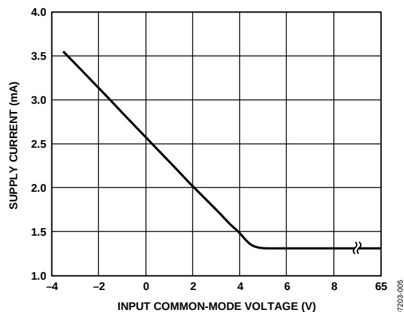
Figure 12. Supply Current vs. Input Common-Mode Voltage
