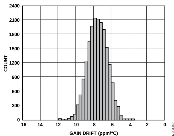
Figure 24. Gain Drift Distribution
