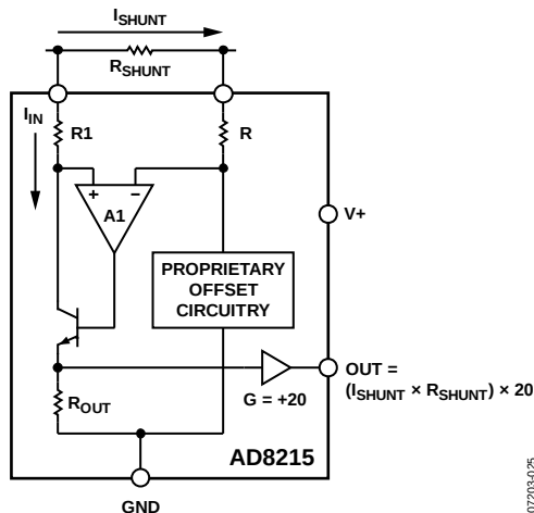
Figure 26. Simplified Schematic
