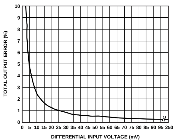
Figure 8. Total Output Error vs. Differential Input Voltage
