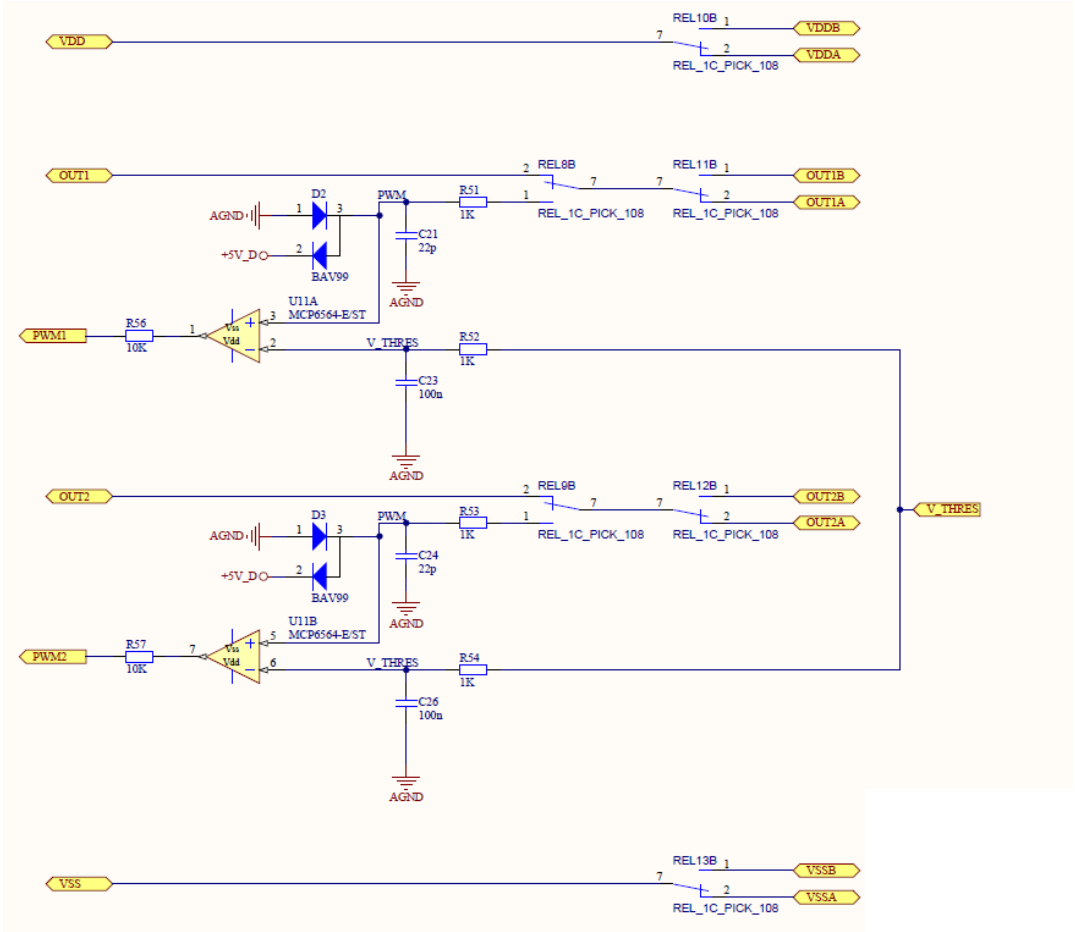
Figure 7: Measure Block
