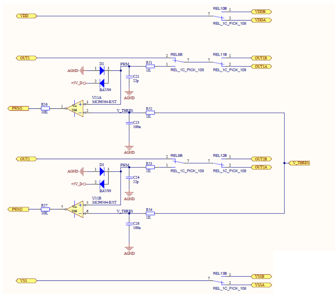
Figure 7: Measure Block
