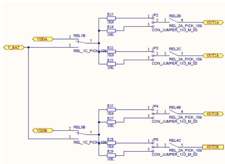
Figure 6: Pull-Up Block
