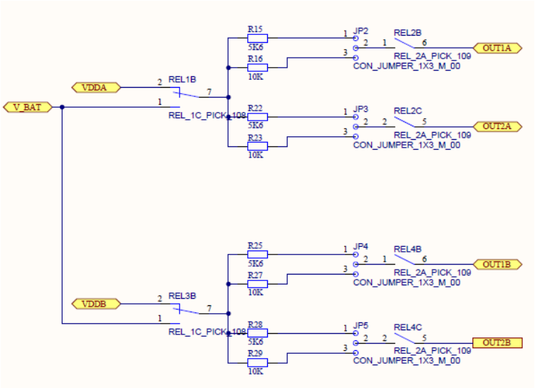
Figure 6: Pull-Up Block
