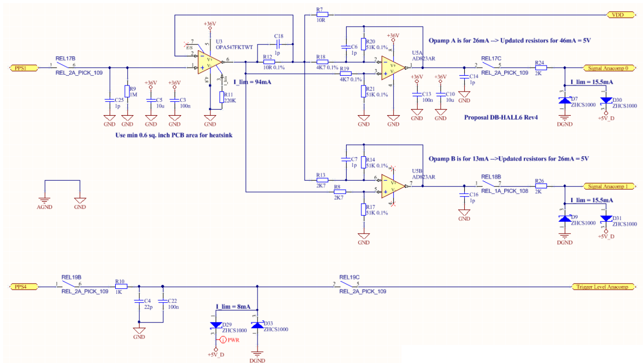
Figure 11: PSI5 Block
