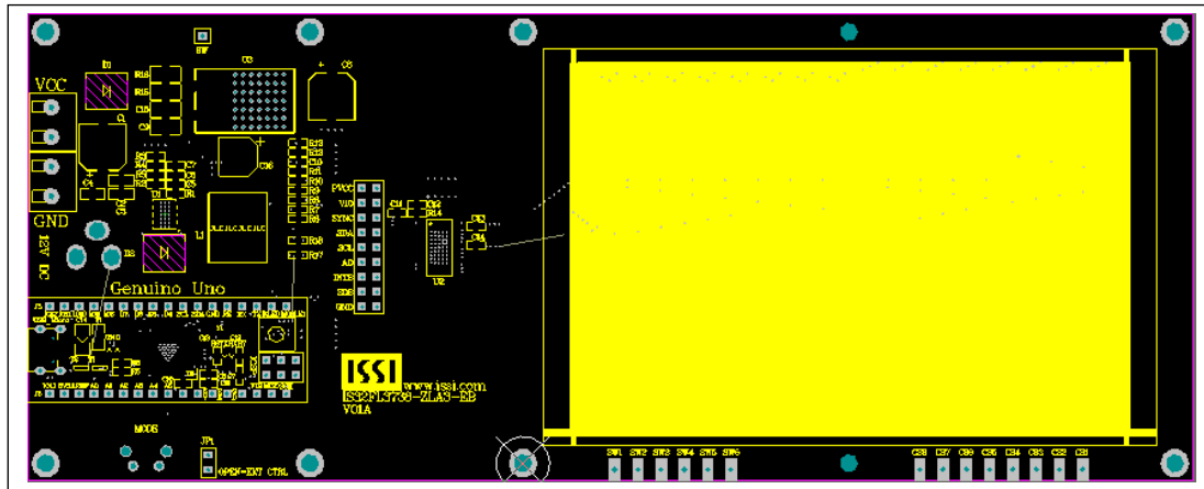
Figure 9: Board Component Placement Guide - Top Layer: V01A
