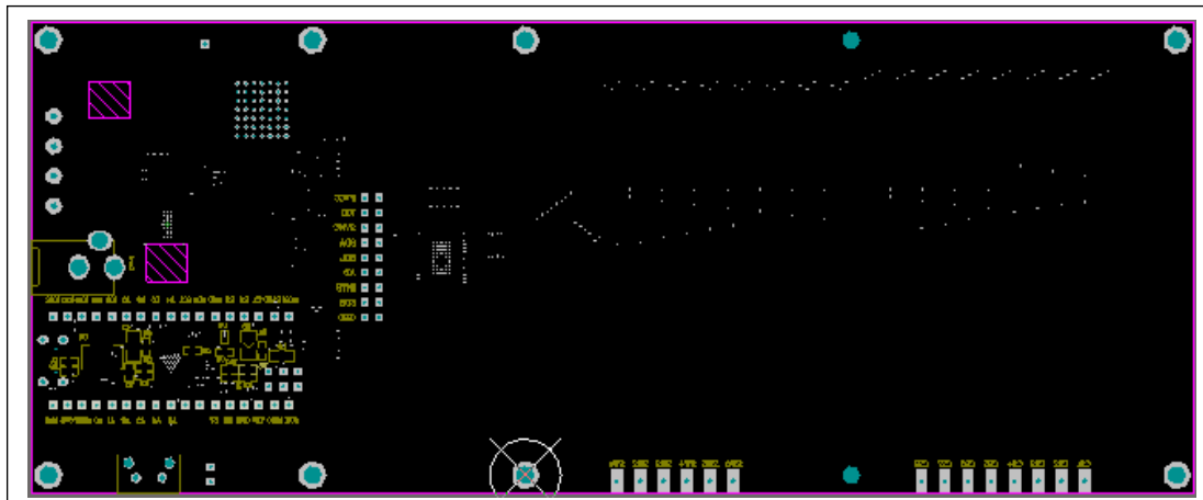
Figure 11: Board Component Placement Guide - Bottom Layer: V01A
