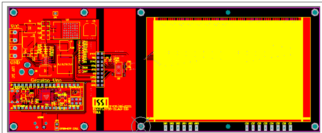
Figure 10: Board PCB Layout - Top Layer: V01A
