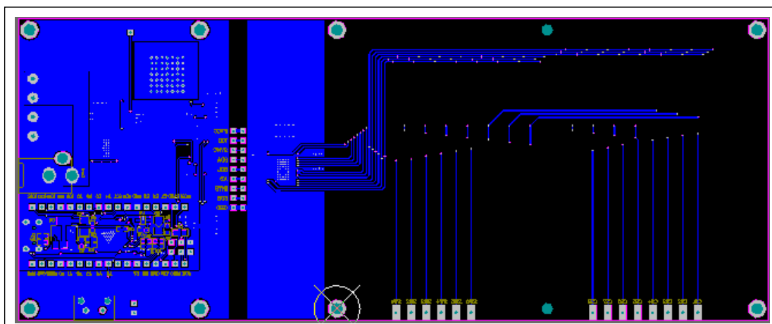
Figure 12: Board PCB Layout - Bottom Layer: V01A
