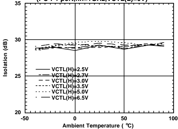
Isolation vs. Ambient Temperature (PC-P1 \text{ port}, f_{in}=1GHz, V_{CTL(L)}=0V)
