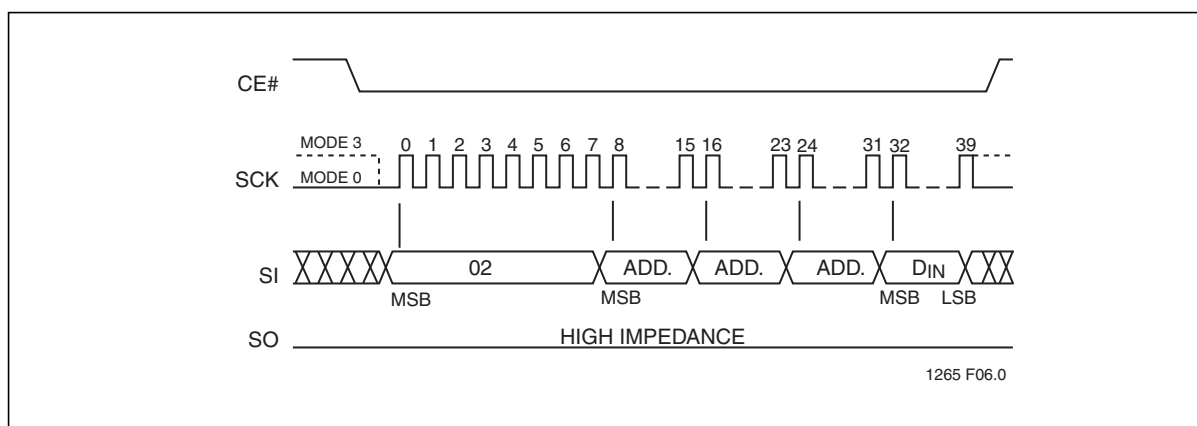
Figure 6: Byte-Program Sequence
