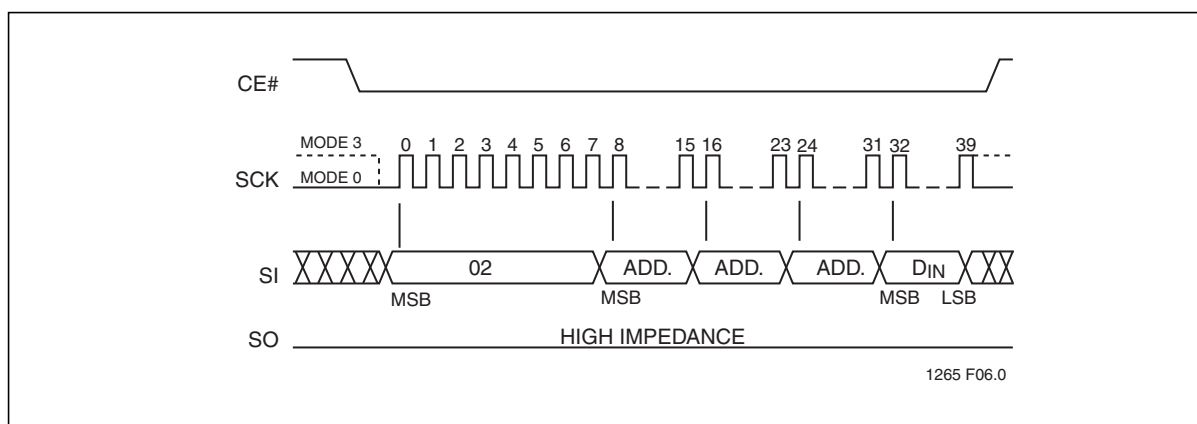
Figure 6: Byte-Program Sequence
