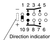
1-coil latching
