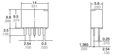
Self-clinching terminal
