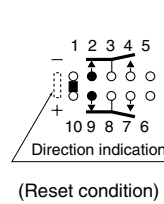
1-coil latching
