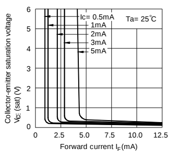
Fig.3 Collector-emitter Saturation Voltage vs. Forward Current
