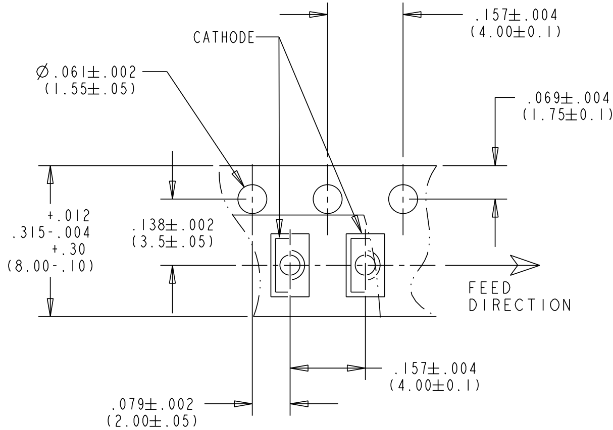
TAPING SPECIFICATION NO SCALE
