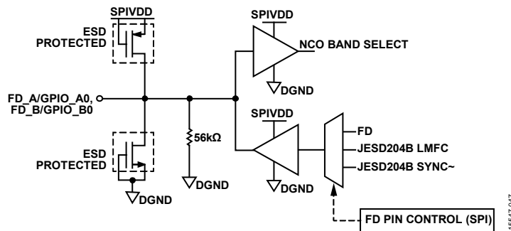
Figure 51. FD_A/GPIO_A0, FD_B/GPIO_B0
