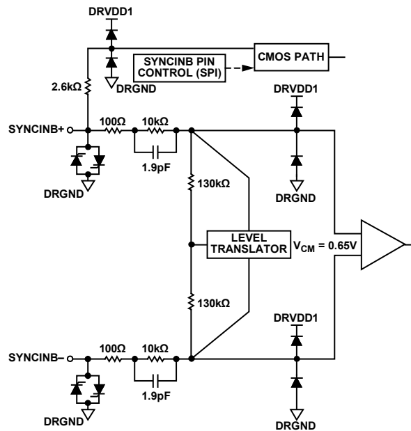
Figure 45. SYNCINB\pm Inputs
