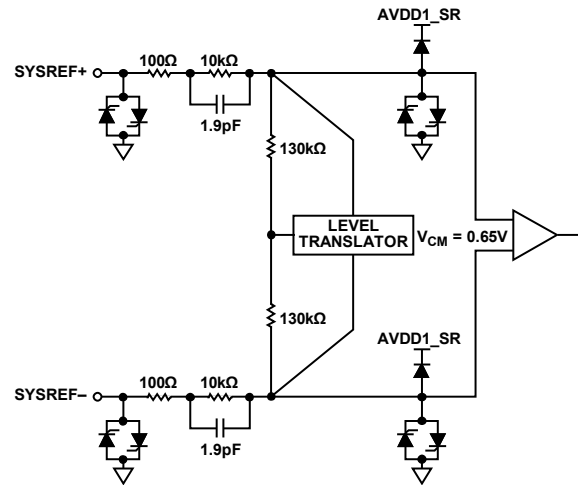
Figure 43. SYSREF\pm Inputs
