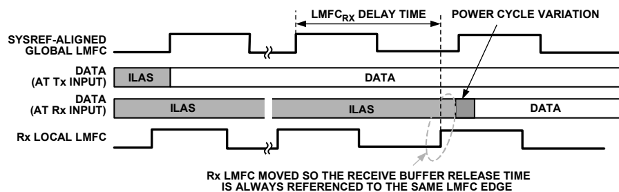
Figure 120. Adjusting the JESD204B Rx LMFC in the Logic Device
