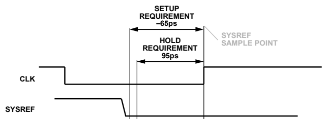
Figure 125. SYSREF High to Low Transition Using Rising Edge Clock Capture (Register 0x0120, Bit 4 = 1'b1; Register 0x0120, Bit 3 = 1'b0)
