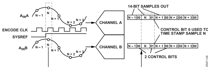
Figure 121. AD9208 Timestamping Example—CS = 2 (Register 0x058F, Bits[7:6] = 2), Control Bit 0 is SYSREF (Register 0x0559, Bits[3:0] = 5)
