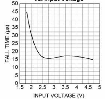
MIC94072/73 Fall Time vs. Input Voltage
