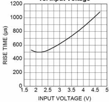
MIC94072/73 Rise Time vs. Input Voltage
