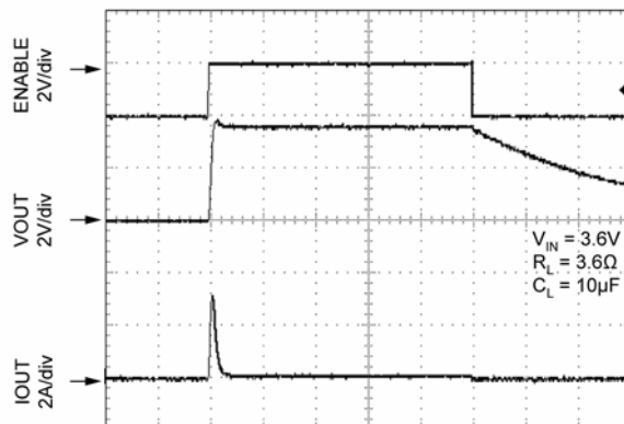
TIME 100µs/div
