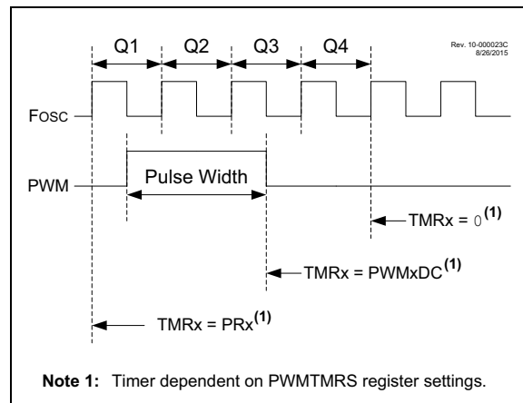
FIGURE 30-1: PWM OUTPUT
