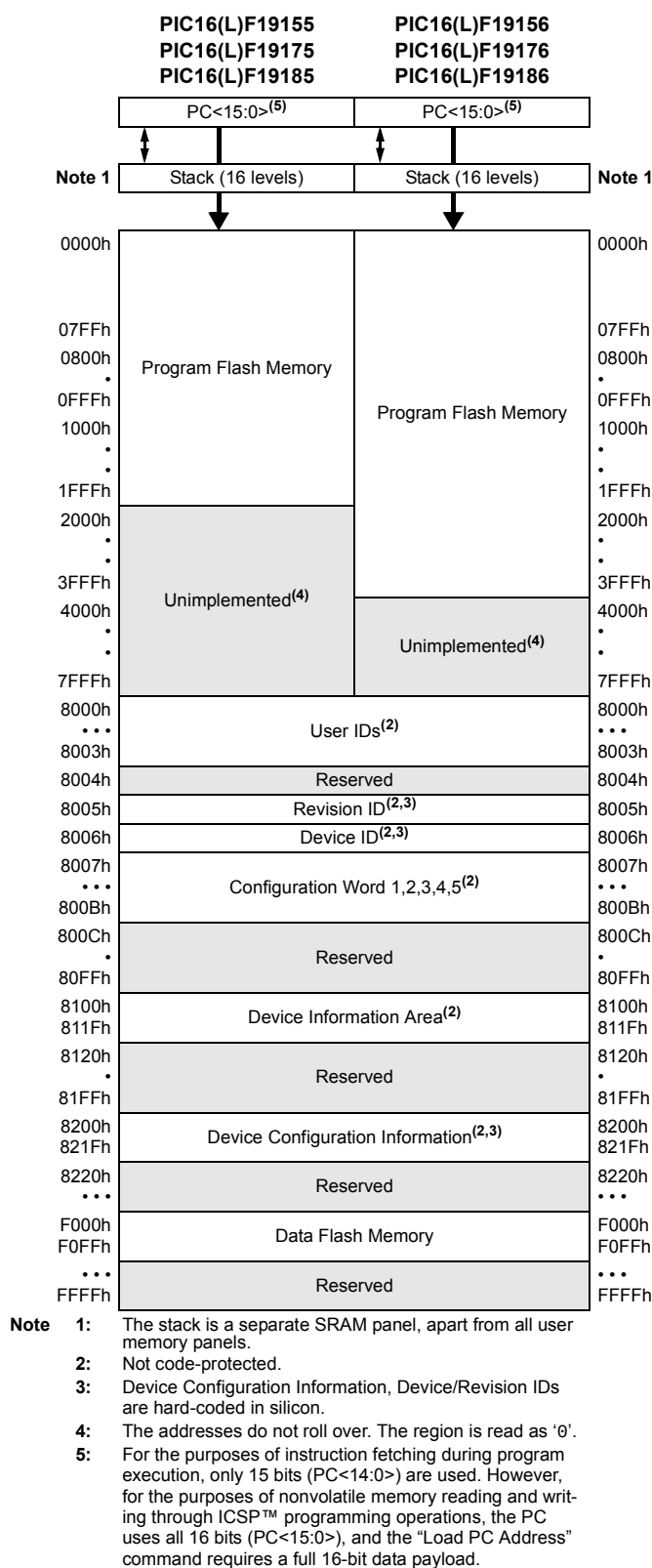
FIGURE 4-1: PROGRAM MEMORY MAP AND STACK FOR PIC16(L)F19155/56/75/76/85/86
