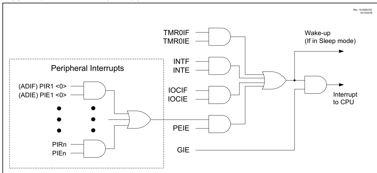
FIGURE 10-1: INTERRUPT LOGIC
