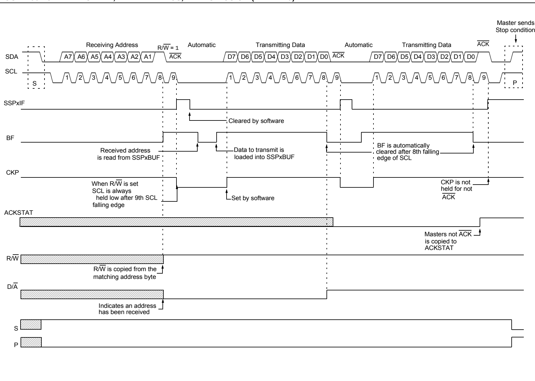
FIGURE 33-18: I 2 C SLAVE, 7-BIT ADDRESS, TRANSMISSION (AHEN = 0)
