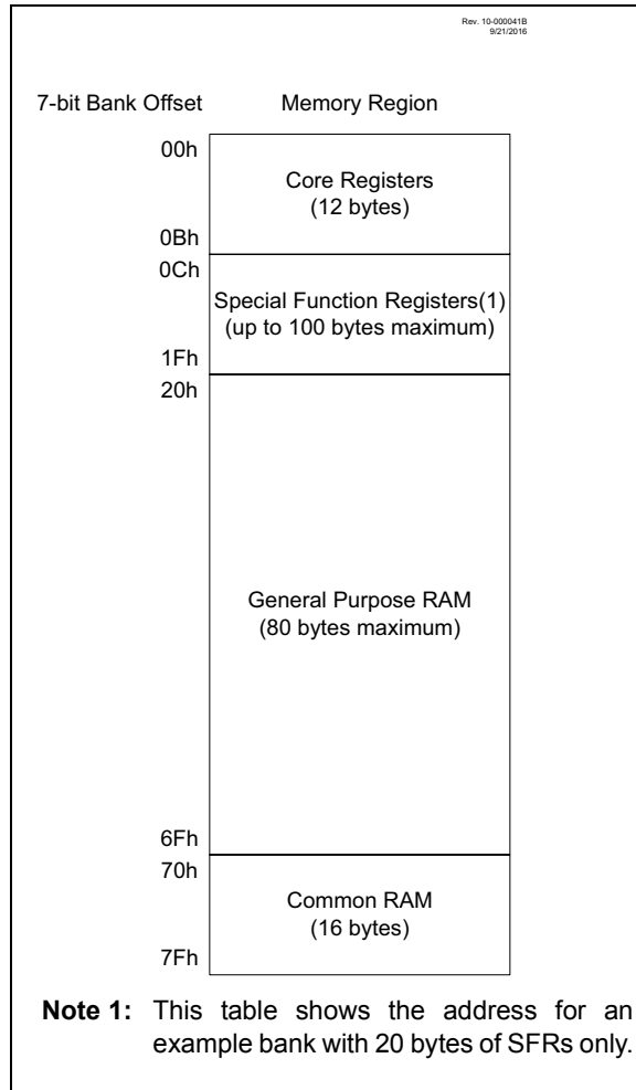
FIGURE 4-2: BANKED MEMORY PARTITIONING
