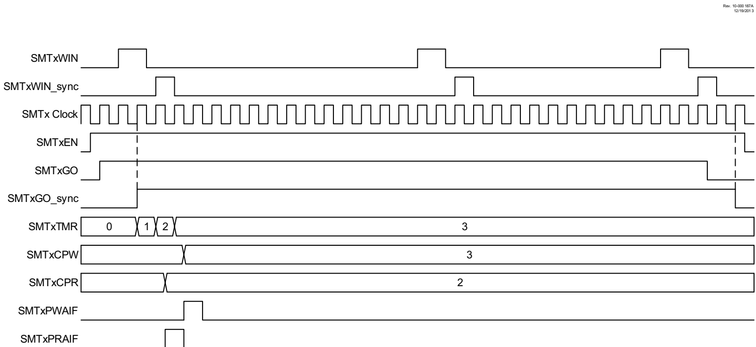
FIGURE 28-17: CAPTURE MODE SINGLE ACQUISITION TIMING DIAGRAM
